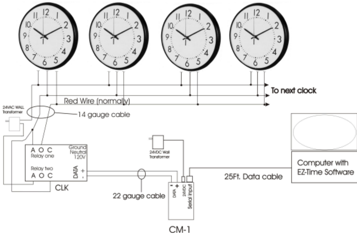
WIRING DIAGRAM FOR CLK
